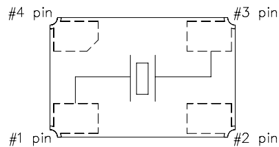
<PIN CONNECTION> TOP VIEW
